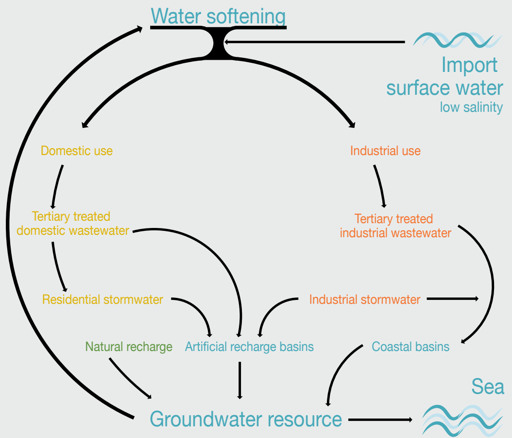
Sequence of operations of the Atlantis Water Resources Management Scheme
